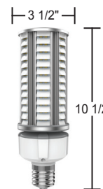
LCE39-54C-DS Dark Sky LED Lamp 54Watt, 4000K, 5900lm Replaces up to 250W MH 180° Down Beam Angle
