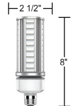
LCE39-24C-DS Dark Sky LED Lamp 24Watt, 4000K, 2400lm Replaces up to 100W MH 180° Down Beam Angle
