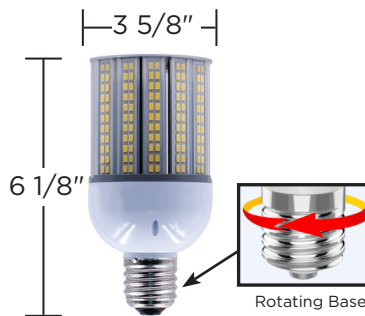
LCE39-20C-T3 Type 3 LED Lamp 20 Watt, 4000K, 3000lm Replaces up to 100W MH 180° Adjustable Beam Angle DLC Listed lamp #GKS38-20W [E;EX]39 (4000K)
